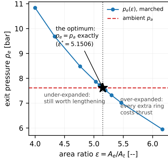
(c) why an optimum exists at all: the exit pressure crosses the ambient
