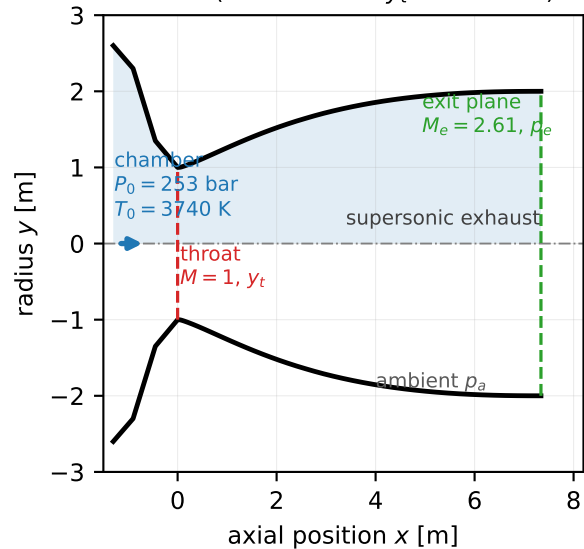
(a) the machine: a converging--diverging nozzle (throat radius y_t = 1 m here)
