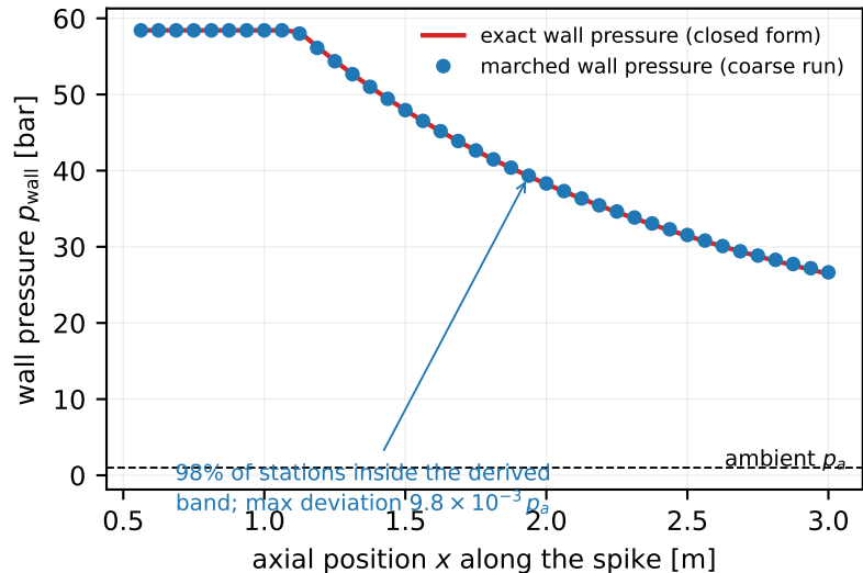
(b) the P-2 meter: wall pressure on the closed form
