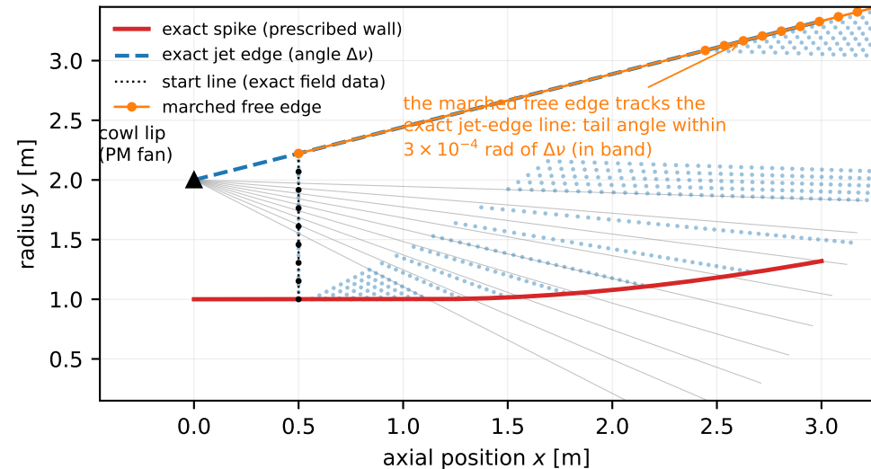
(a) the certified march in the oracle world
