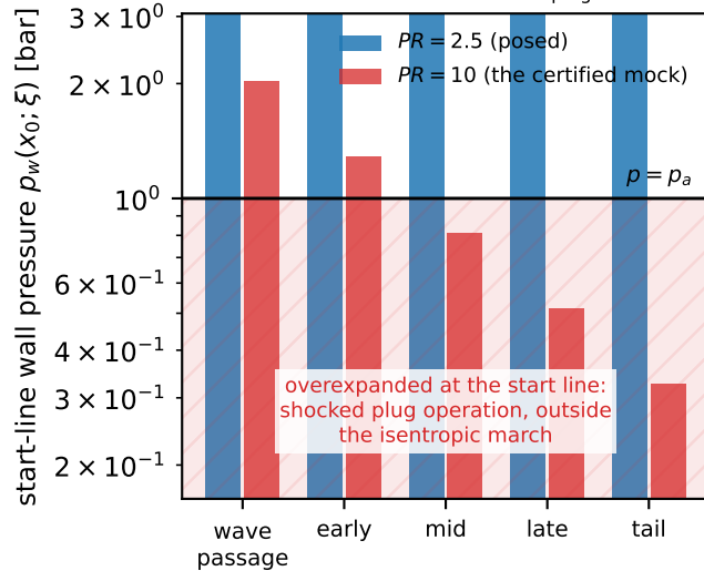
(b) the plug feels the ambient: the shock-free bound PR_{\text{plug}} = 2.5
