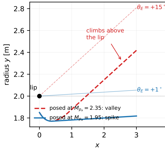
(a) the valley spike: fan turned past axial vs the \theta_E \approx 0 posing
