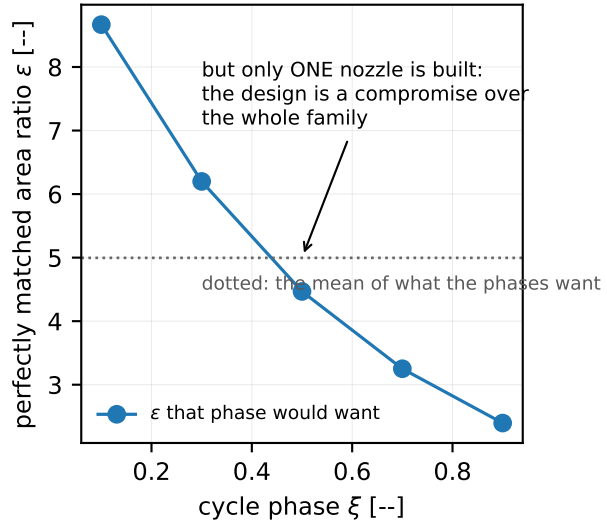
(c) the design problem the cycle creates: five phases, one piece of hardware
