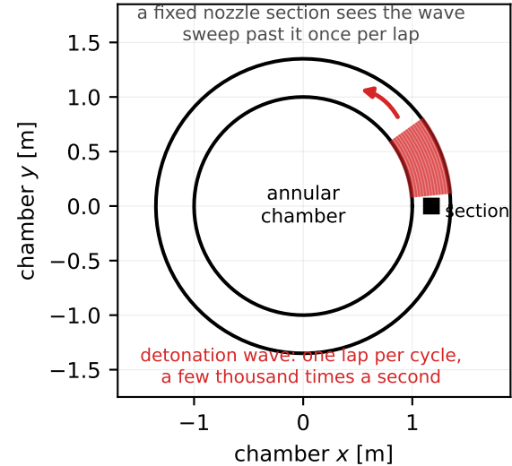
(a) the source of the cycle: a detonation wave rotating in an annulus
