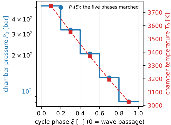
(b) what the nozzle is handed: a periodic family of chamber states (the mock cycle)
