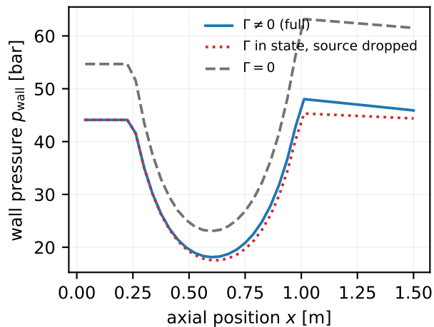
(b) the expansion world: the two alive controls --- swirl and its source both matter
