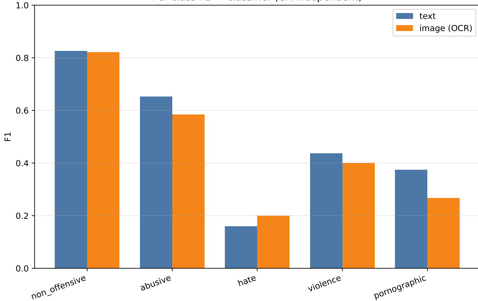
Per-class F1 — classifier (CA-independent)
