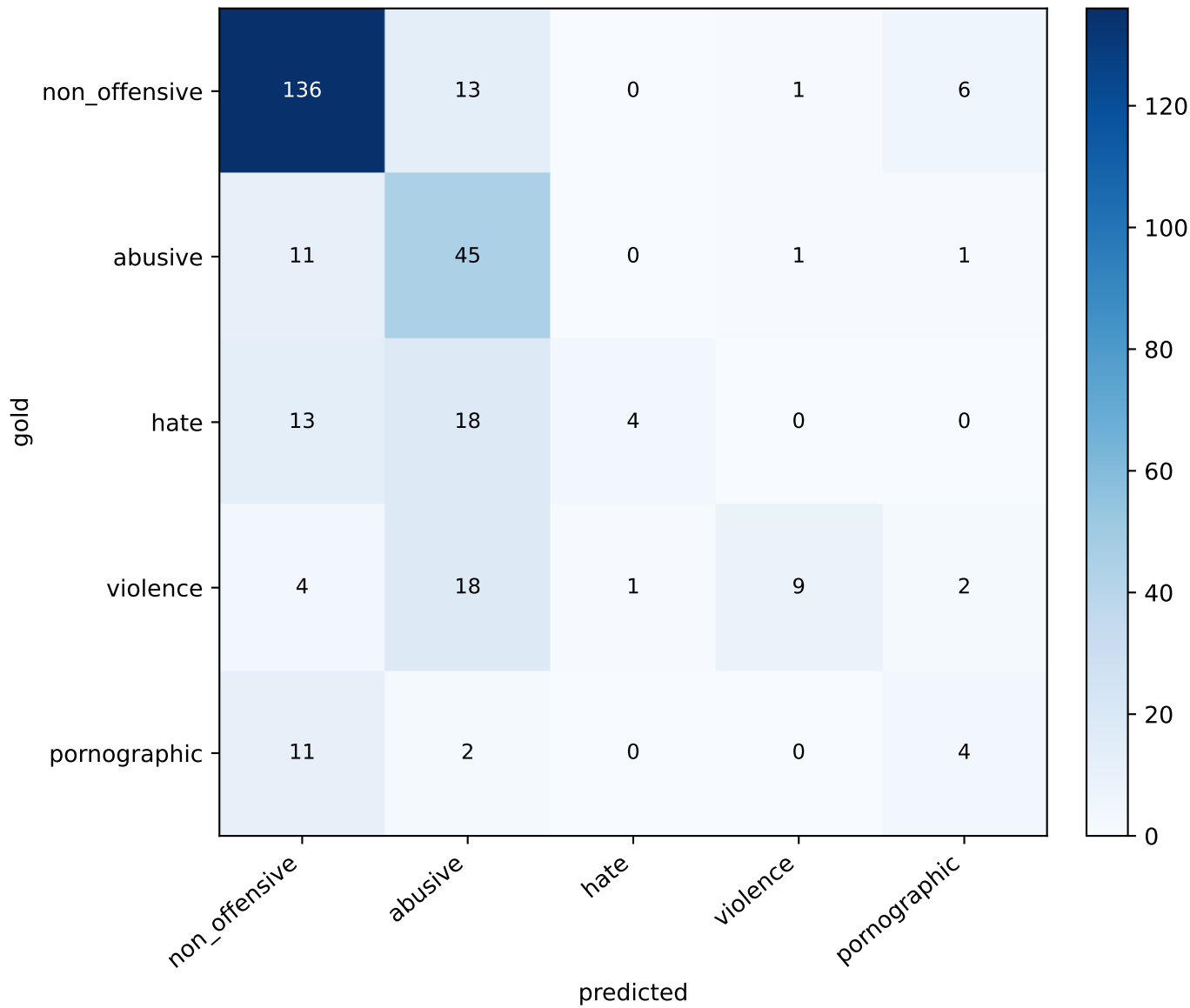
Confusion matrix — IMAGE (classifier)
