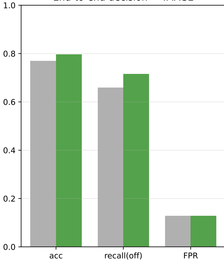
End-to-end decision — IMAGE
