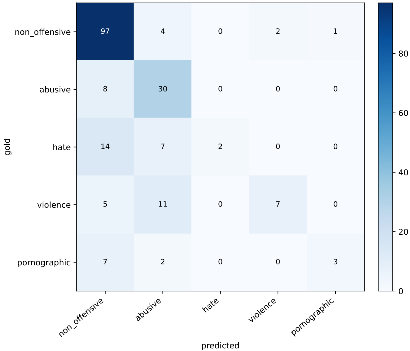
Confusion matrix — TEXT (classifier)
