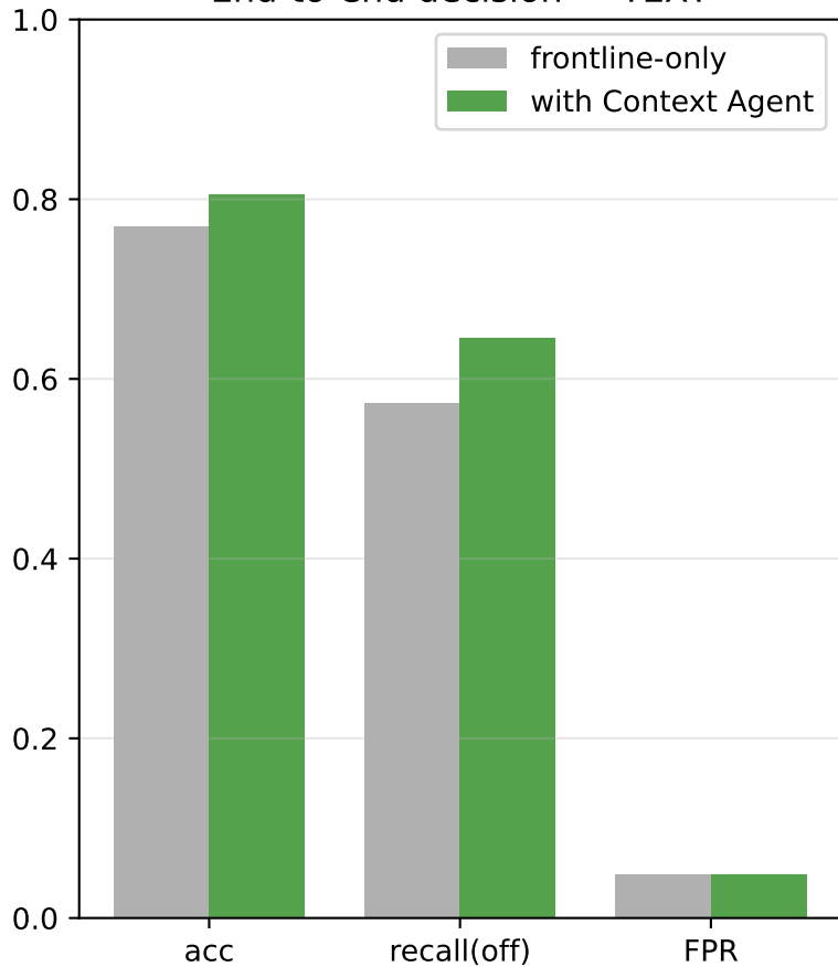
End-to-end decision — TEXT
