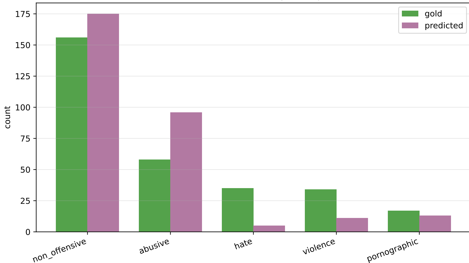
Label distribution — IMAGE (gold vs predicted)
