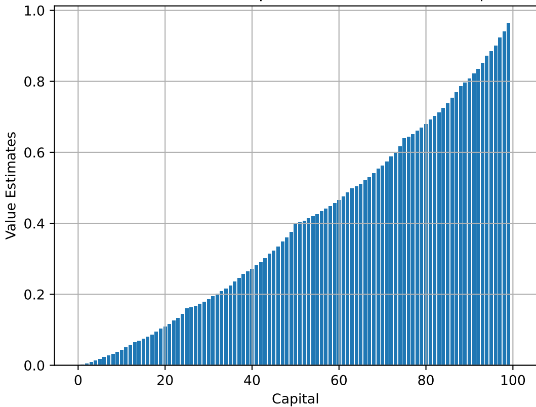
Final value function (expected return) vs State (Capital)
