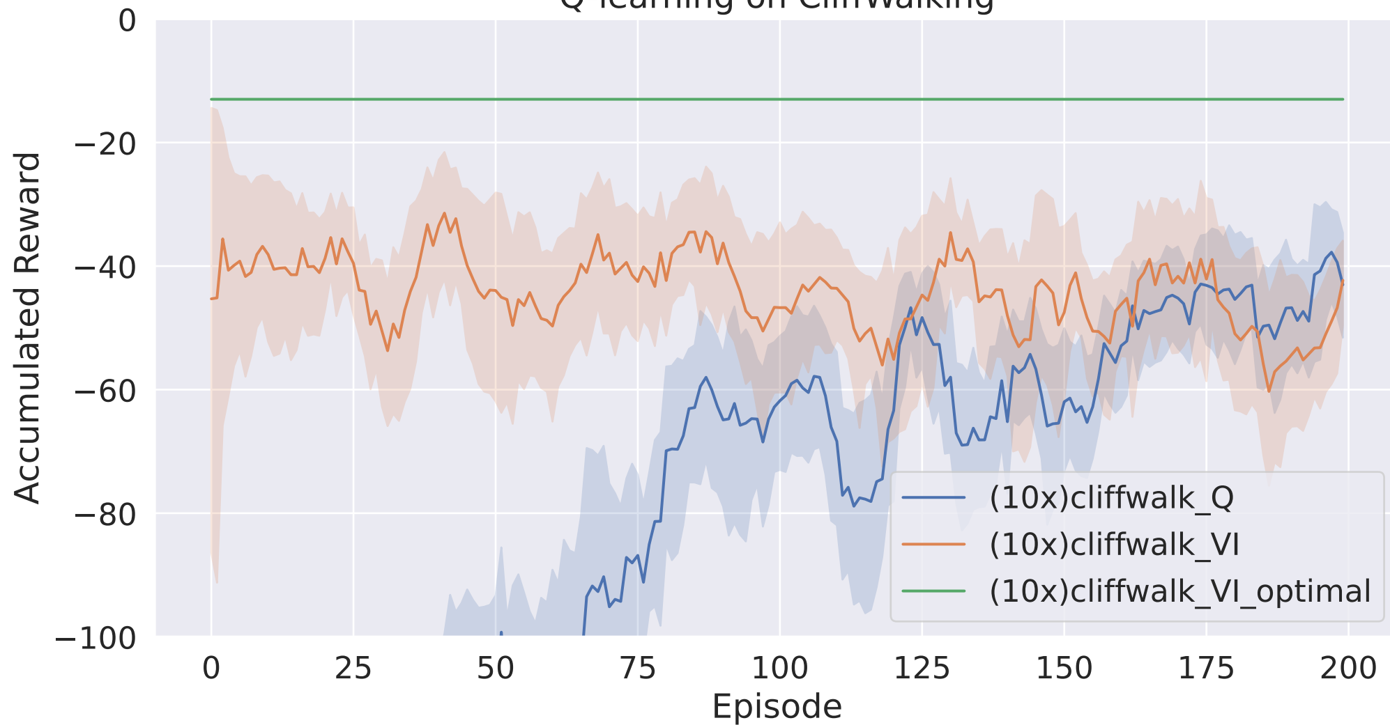
Q-learning on CliffWalking
