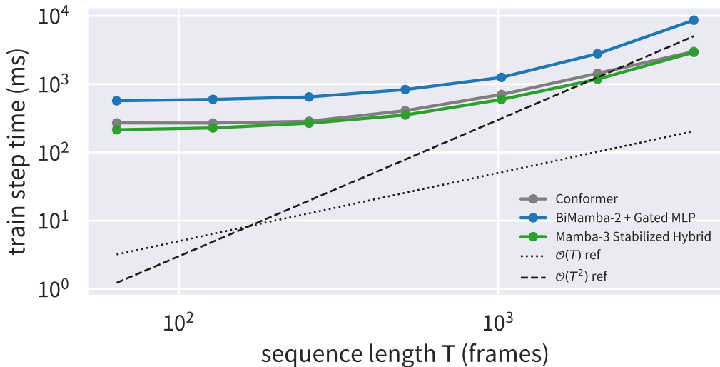
Latency scaling probe (CPU, batch 2, 306 ch)
