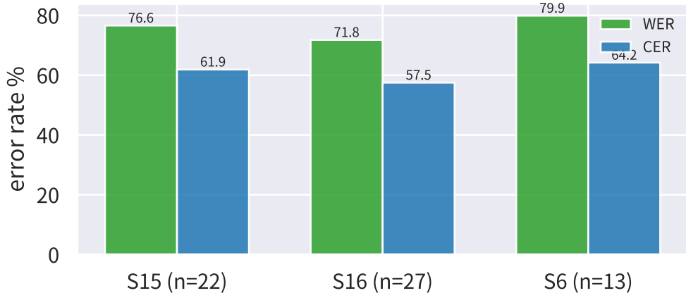
Mamba-3 Stabilized Hybrid — per-subject breakdown
