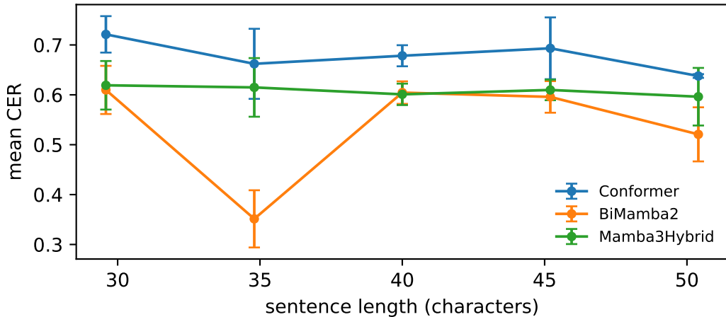
CER vs sentence length
