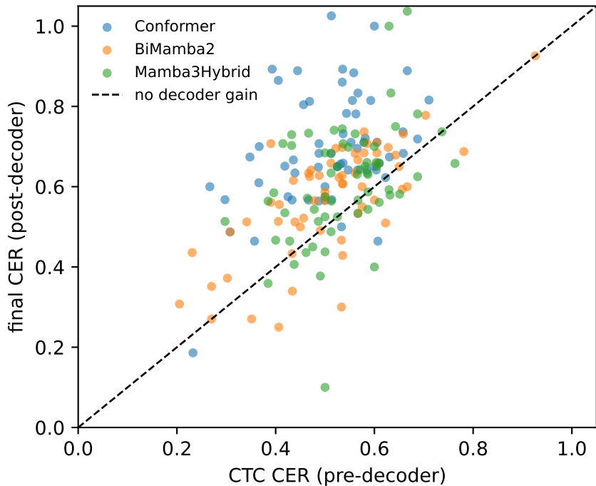
Decoder gain per sentence
