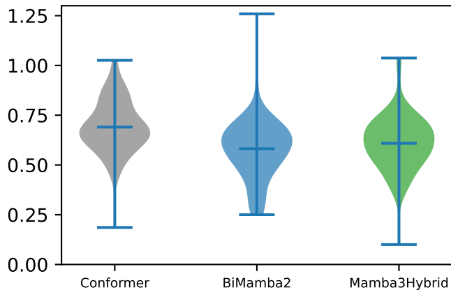
per-sentence CER
