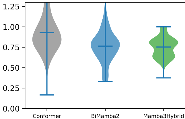
per-sentence WER
