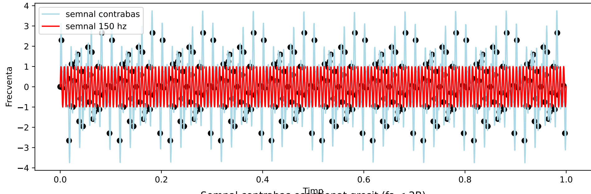
Semnal contrabas esantionat gresit ( f_s < 2B )
