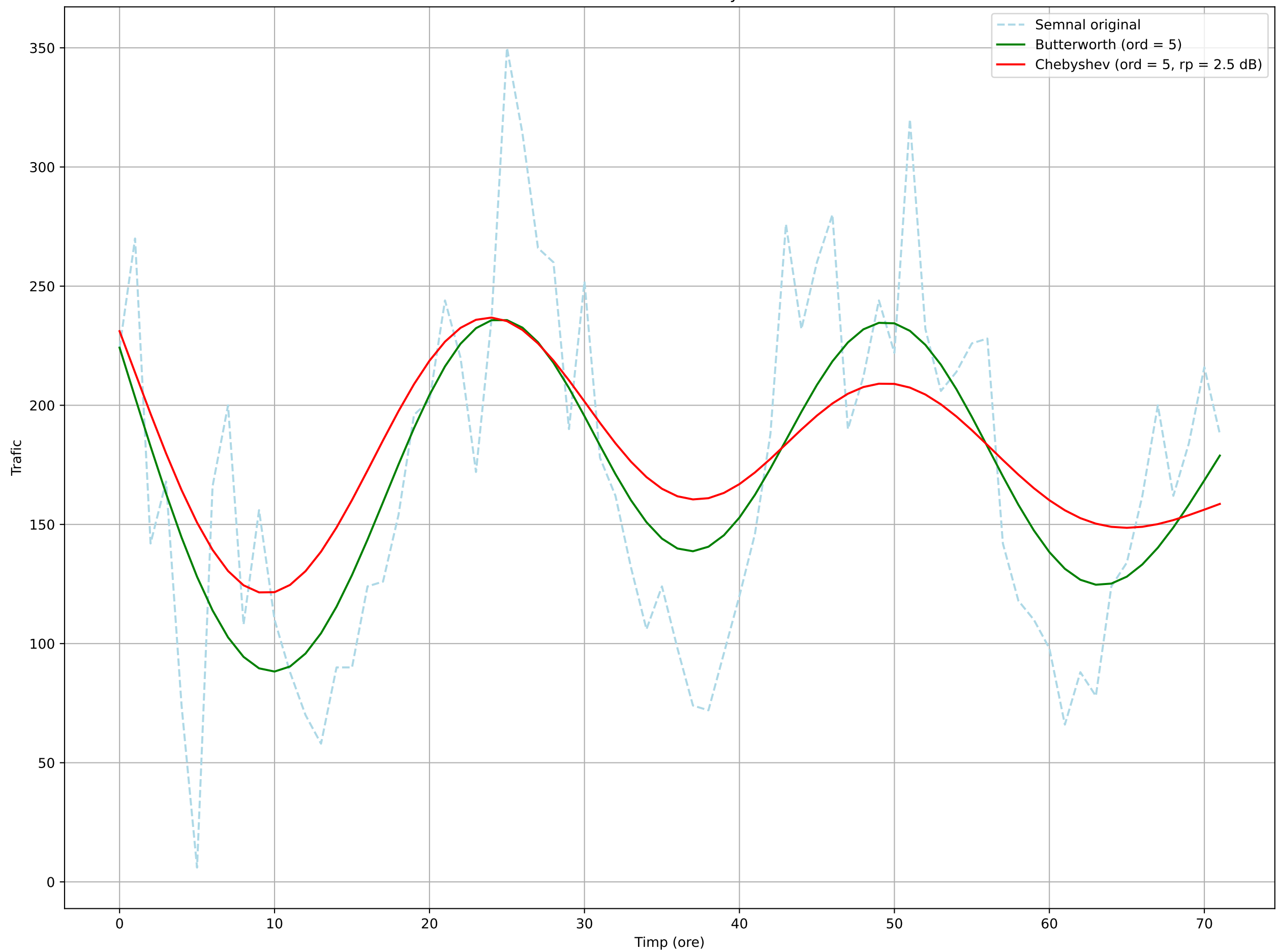
Butterworth vs Chebyshev
