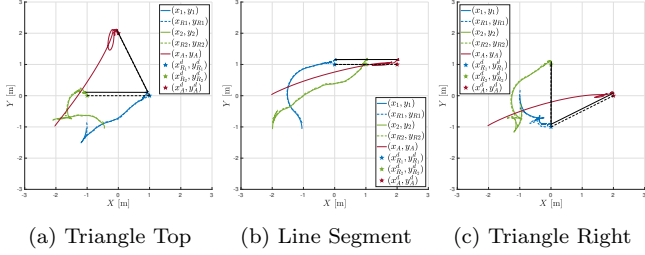
Fig. 10. Trajectories of the three agents with desired and actual interdistances in the experiments with the ground clear of obstacles.
