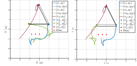
Fig. 11. Trajectories of the three agents with desired and actual interdistances in the experiments with static obstacles.
