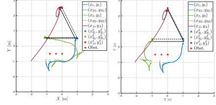
Fig. 11. Trajectories of the three agents with desired and actual interdistances in the experiments with static obstacles.
