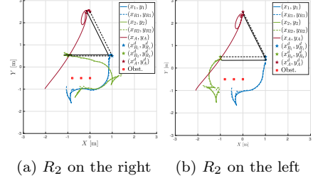
Fig. 9. Trajectories of the three agents with desired and actual interdistances in the experiments with static obstacles.
