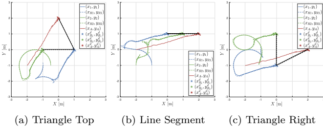
Fig. 7. Trajectories of the three agents with desired and actual interdistances in simulation with disturbances.
