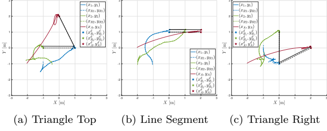
Fig. 8. Trajectories of the three agents with desired and actual interdistances in the experiments with the ground clear of obstacles.
