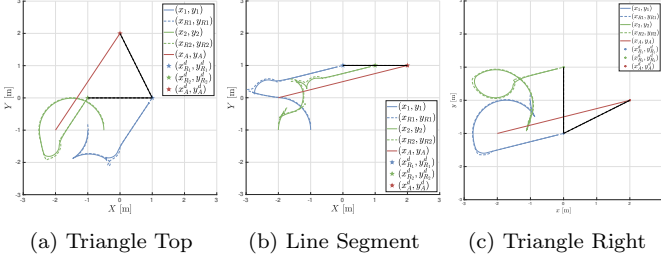
Fig. 5. Trajectories of the three agents with desired and actual interdistances in ideal simulations.
