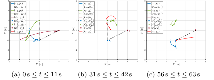
Fig. 10. Trajectories of the three agents with desired and actual interdistances in the experiments with a dynamic obstacle.
