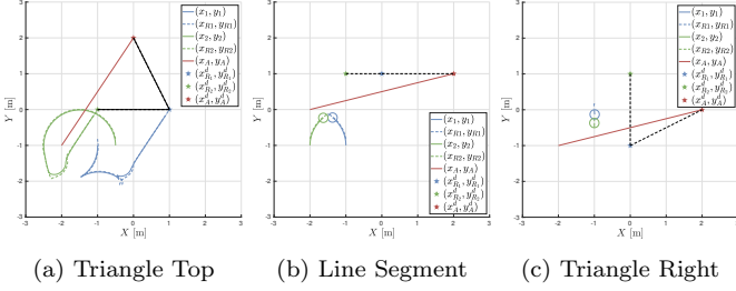
Fig. 6. Trajectories of the three agents without APFs in ideal simulations.
