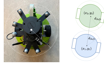
Fig. 4. The physical robot is contained entirely in a circle of radius d_{safe} = 0.13 \text{ m} . Consequently, if the centers of rotation are at a distance less than 2d_{safe} it means that the agents collided.
