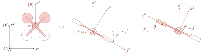
Fig. 3. Quadcopter's roll \phi and pitch \theta angles.
