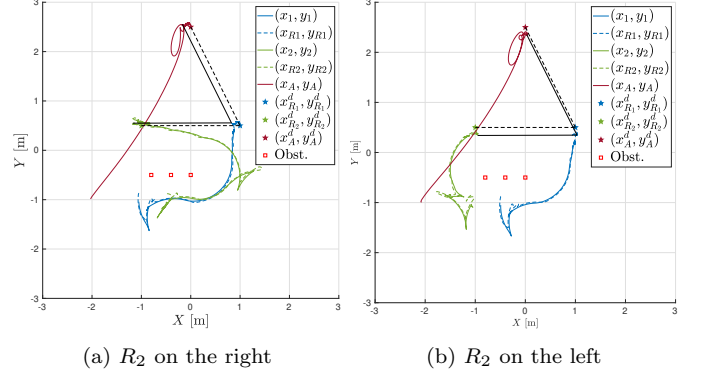
Fig. 10. Trajectories of the three agents with desired and actual interdistances in the experiments with static obstacles.
