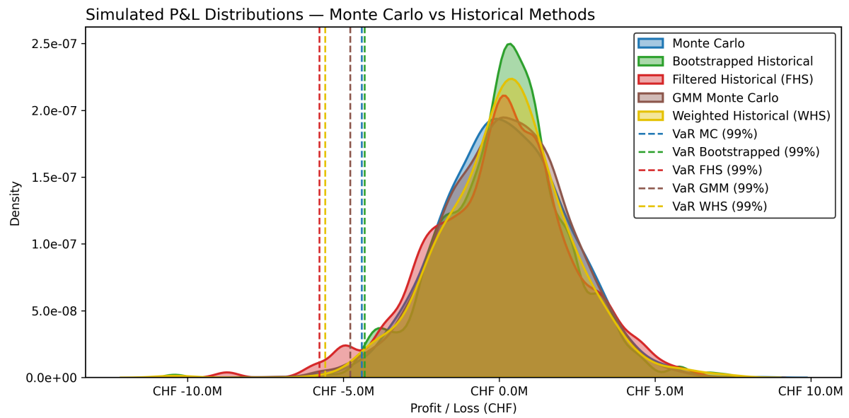
Figure 5: Kernel density estimates of simulated profit and loss with 1-day VaR for each simulation method.
