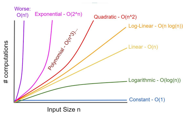
Figura 13.1: O(1) < O(\log n) < O(n) < O(n \log n) < O(n^2) < O(n^3) < \dots < O(a^n)
