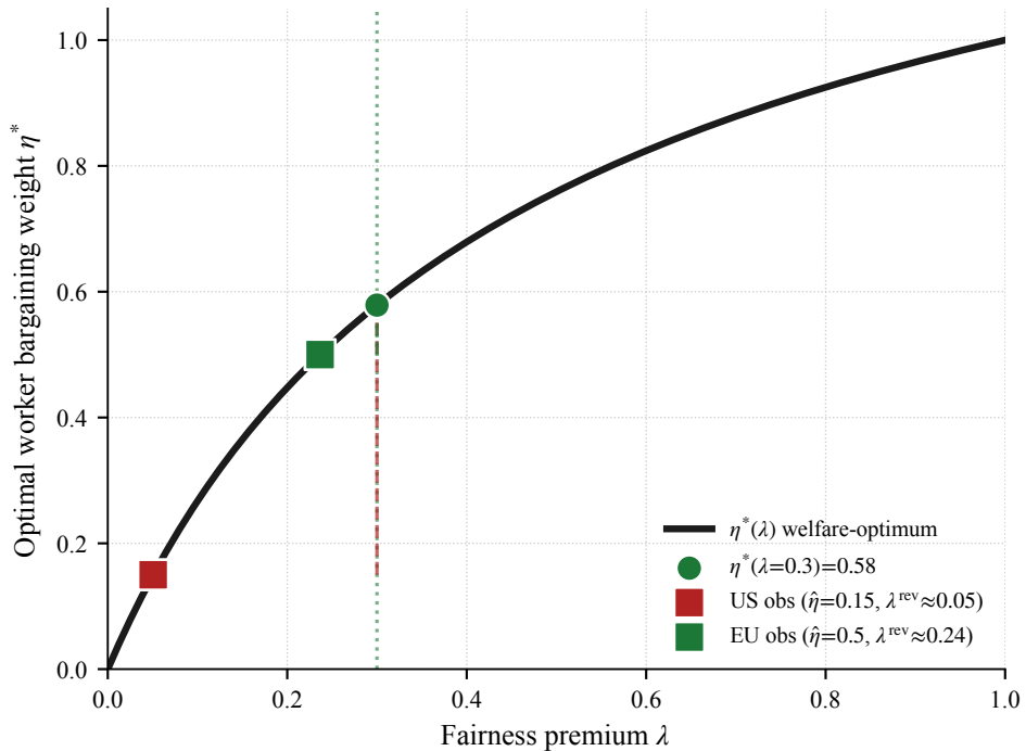
(a) \eta^*(\lambda) : revealed vs. \ common- \lambda readings
