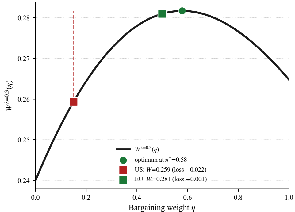
(b) Reading A welfare loss at common \lambda=0.3
