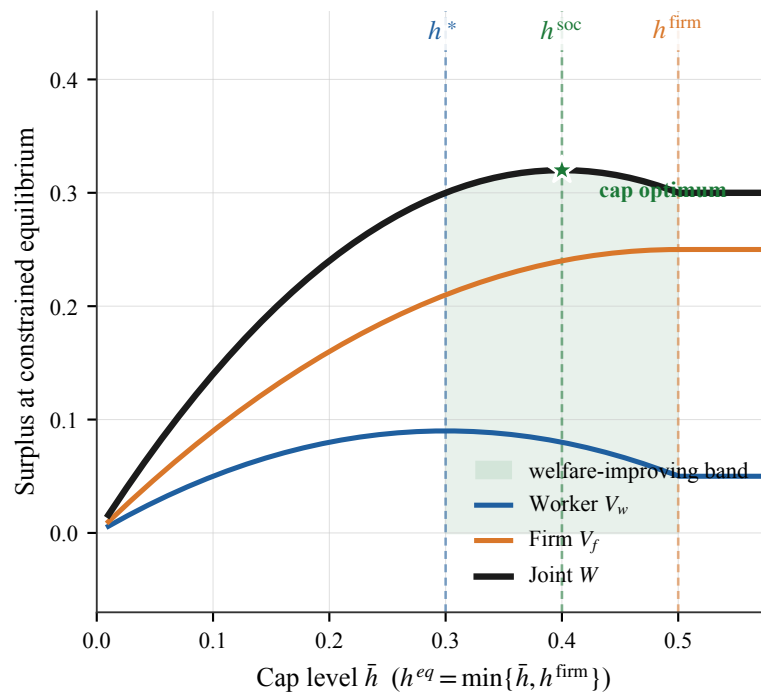
(b) Surplus along h^{eq}(\bar{h})
