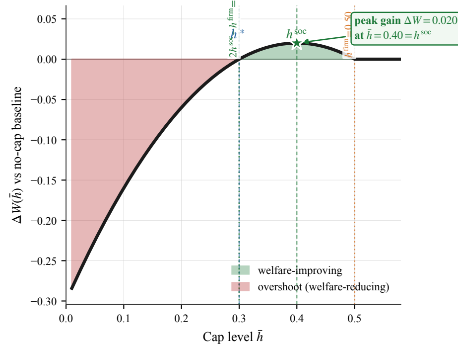
(c) Welfare gain: improving band vs overshoot
