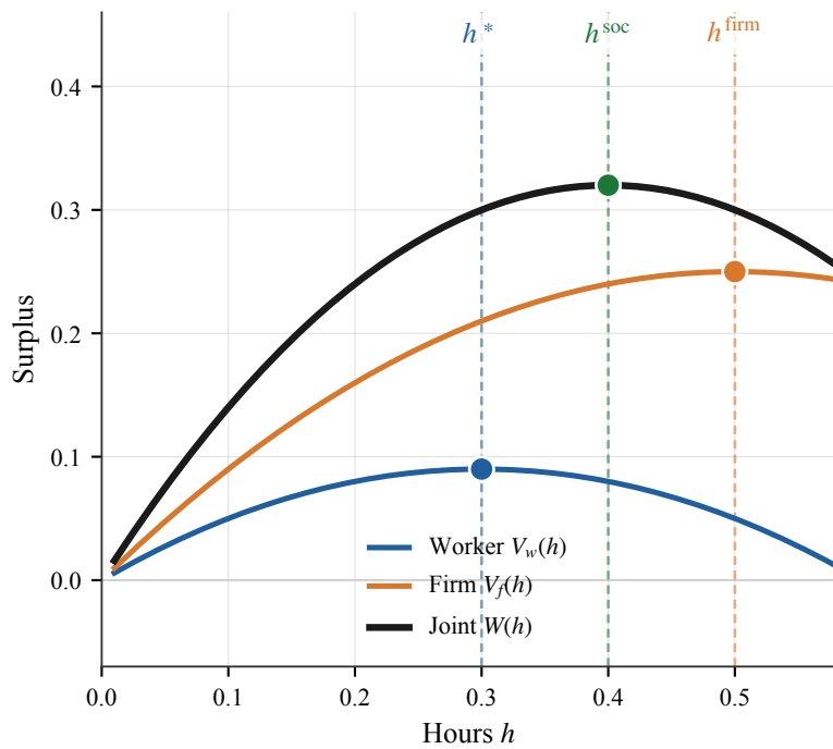
(a) Primitives and bliss points
