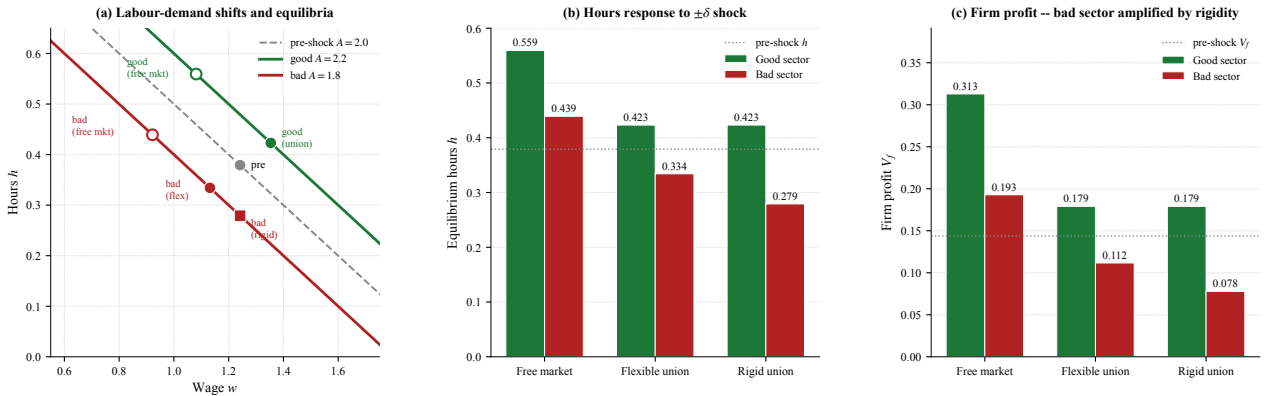
Figure 6: Asymmetric productivity shocks under union wage rigidity. Pre-shock (A, w, h) = (2, 1.242, 0.379) at \eta = 0.5 ; shock \delta = 0.2 . (a) Labour-demand shifts and equilibria across the three regimes (free market, flexible union, rigid union); rigid bad-sector equilibrium sits on the new demand curve at the stuck pre-shock wage. (b) Hours response: good sector rises under all regimes, bad sector rigidity is 36% below free market. (c) Firm profit: bad sector under rigidity is 60% below free market. Source: sim_models_v2.py:make_shocks .
