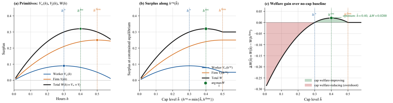
Figure 3: Hours-cap simulation. (a) primitives V_w , V_f , W over h with interior maxima marked; (b) surplus along h^{\text{eq}}(\bar{h}) = \min\{\bar{h}, h^{\text{firm}}\} ; (c) \Delta W(\bar{h}) vs no-cap baseline – green band is the welfare-improving region of (4), red is overshoot. Maximum gain \Delta W = 0.020 at \bar{h} = h^{\text{soc}} = 0.40 . Source: sim_mechanisms.py .
