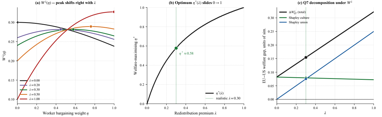
Figure 5: Welfare under Saez–Stantcheva (2016) weights. (a) W^\lambda(\eta) for \lambda \in \{0, 0.2, 0.3, 0.5, 1\} : peak shifts right with \lambda . (b) \eta^*(\lambda) : realistic \lambda=0.30 (HSV 2017 + log utility) gives \eta^* \approx 0.58 , consistent with European RTM coverage of 80–95%. (c) Q7 EU–US gap and Shapley decomposition under W^\lambda : at \lambda=0 culture does everything, union nets to zero; at \lambda=0.30 they contribute roughly equally (+0.079 vs +0.076); at \lambda=0.50 union dominates. Source: sim_models.v2.py:make_redistribution.
