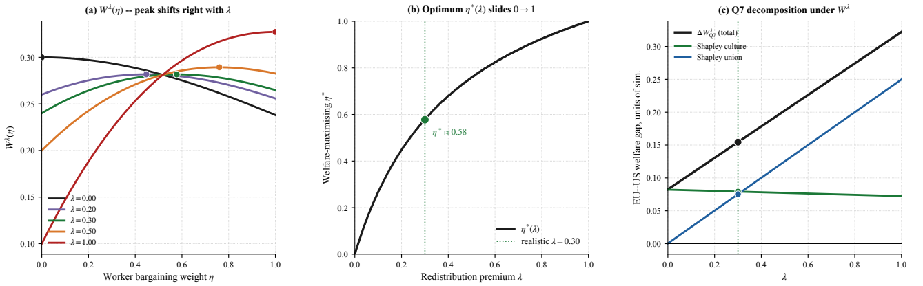
Figure 5: Welfare under Saez–Stantcheva (2016) weights. (a) W^\lambda(\eta) for \lambda \in \{0, 0.2, 0.3, 0.5, 1\} : peak shifts right with \lambda . (b) \eta^*(\lambda) : realistic \lambda=0.30 (HSV 2017 + log utility) gives \eta^* \approx 0.58 , consistent with European RTM coverage of 80–95%. (c) Q7 EU–US gap and Shapley decomposition under W^\lambda : at \lambda=0 culture does everything, union nets to zero; at \lambda=0.30 they contribute roughly equally (+0.079 vs +0.076); at \lambda=0.50 union dominates. Source: sim_models.v2.py:make_redistribution .
