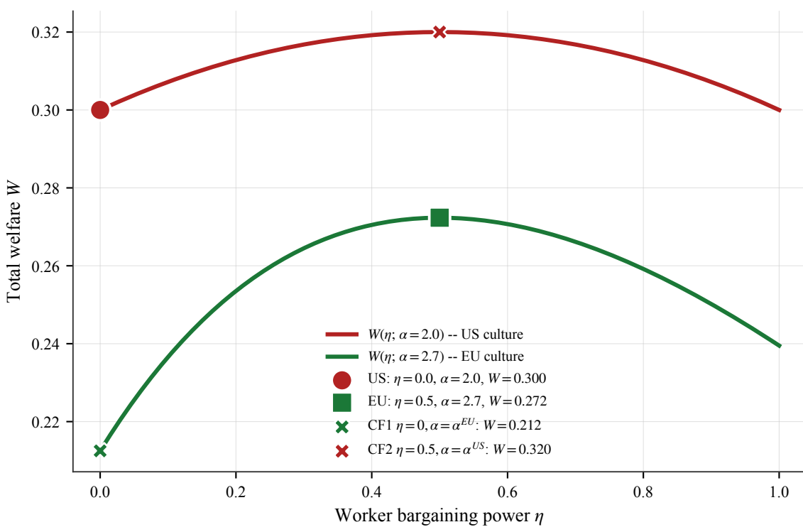
(a) Welfare frontier: W(\eta; \alpha) and US/EU equilibria
