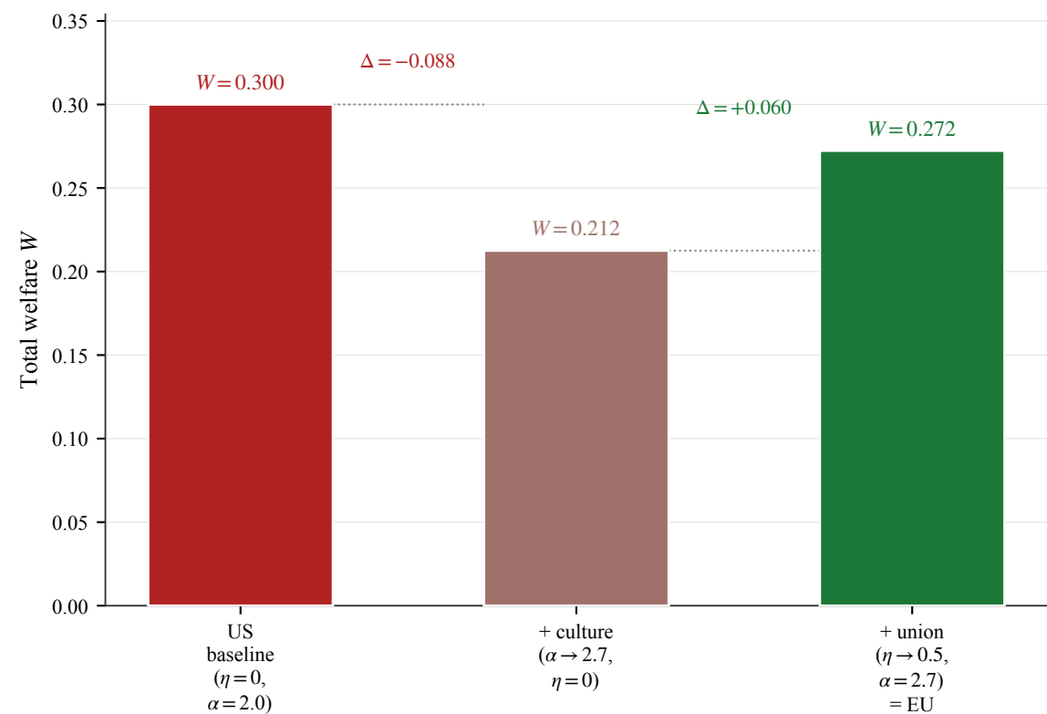
(b) US \rightarrow EU decomposition: which channel costs how much
