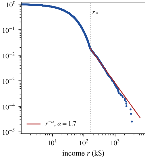
log-log: Pareto tail
