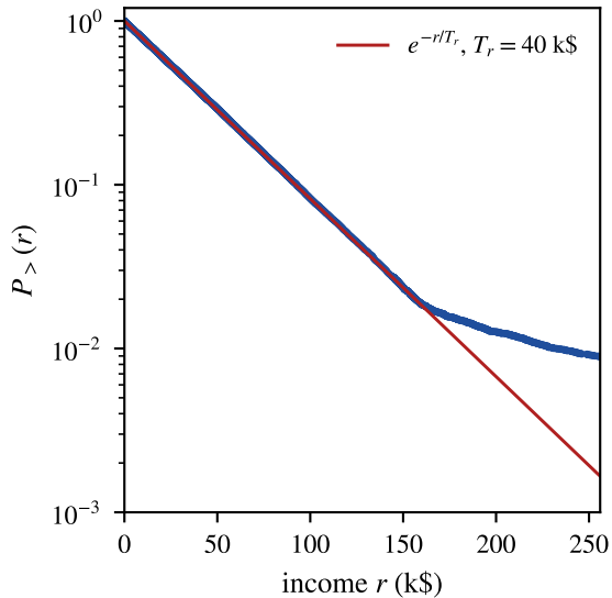
log-linear: Boltzmann bulk
