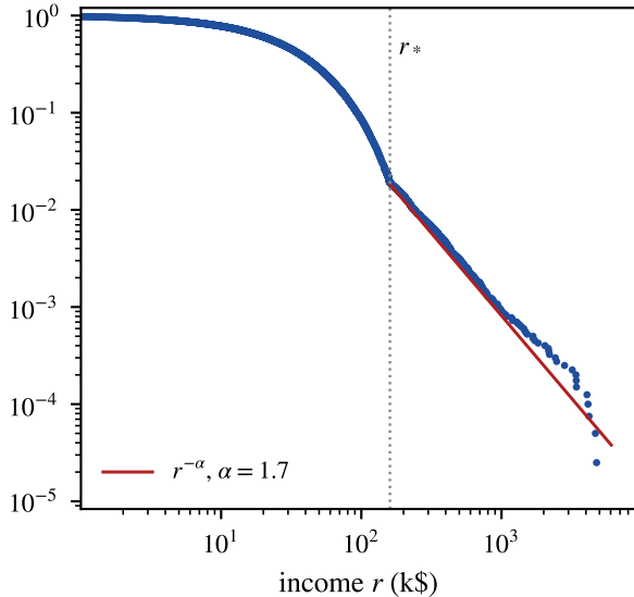
log-log: Pareto tail
