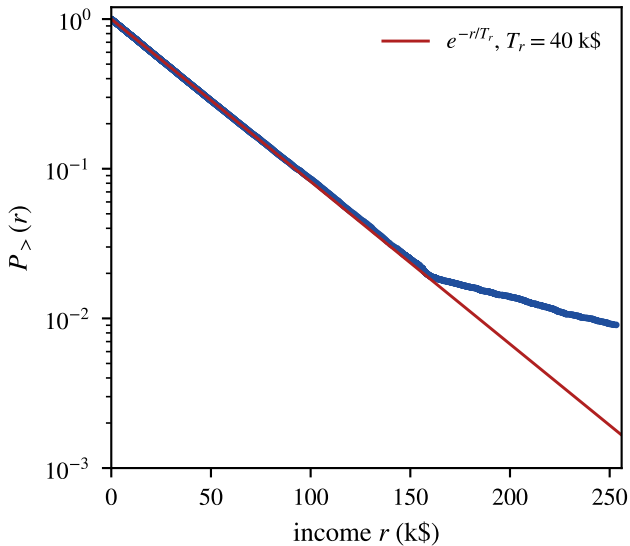
log-linear: Boltzmann bulk
