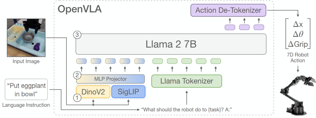
Figure 14: OpenVLA architecture, credits [9]
