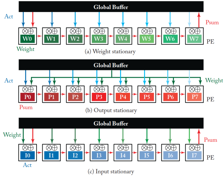
Figure 2: Different dataflow architectures, credits [10]
