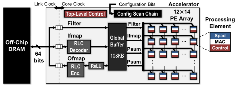
Figure 7: Eyeriss architecture, credits [5]
