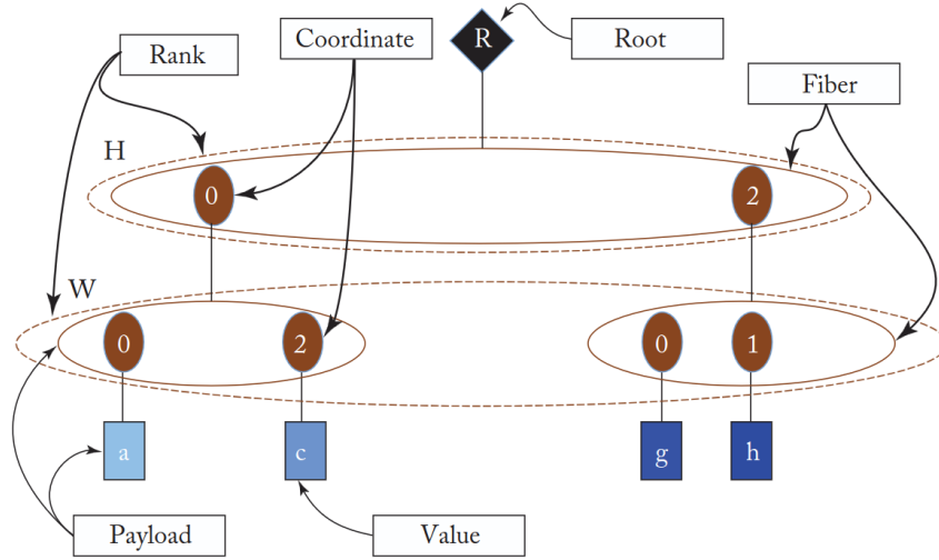
Figure 6: Fiber-tree representation, credits [10]
