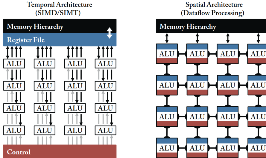
Figure 1: Temporal and Spatial architecture, credits [10]
