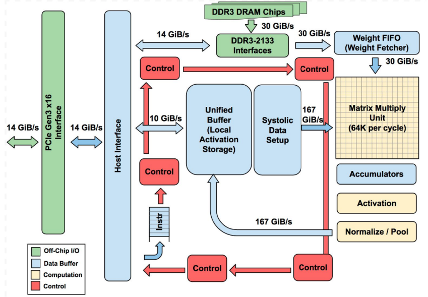
Figure 8: TPU architecture, credits [8]
