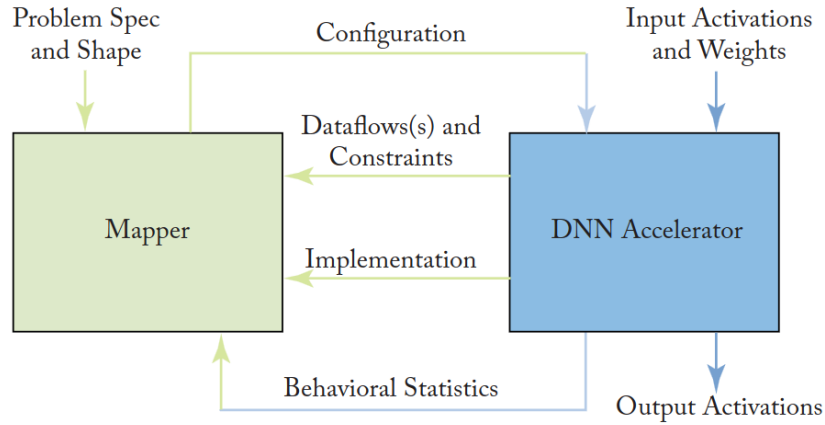
Figure 5: Mapping a DNN model on specialized HW, credits [10]
