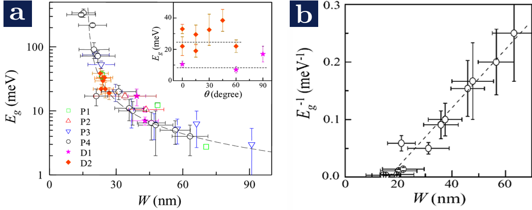
Figure 1.4: (a) E_g vs W for four (P1–P4) of the parallel devices and two (D1, D2) with varying orientation. The inset shows E_g vs relative angle \theta for the device D1 and D2. (b) E_g^{-1} vs W . (c) Conductance vs width of parallel GNRs measured at a gate voltage V - V_g = 50 V. Squares are values measure at 300 K whereas triangle corresponds to 1.6 K. The insets show the conductivity (upper) and the inactive GNR width (lower) obtained from the slope and x intercept of the linear fit at varying temperatures. Adapted from [63].
