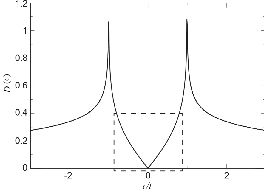
Figure 1.1: Graphene density of states plotted over a wide range of nearest neighbor hopping parameter t , showing pronounced van Hove singularities for \epsilon \sim \pm t [castroneto2009]. The dashed rectangle indicates the almost linear low energy DOS normally spanned in back-gated transport measurements.
