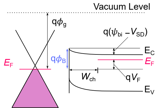
Forward bias
