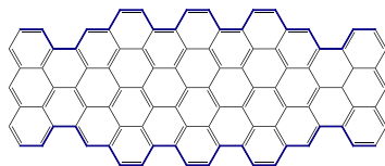
heterojunction
