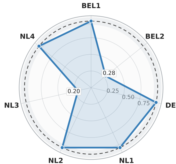
a) Grid connection capacity
