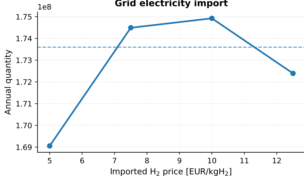
Grid electricity import
