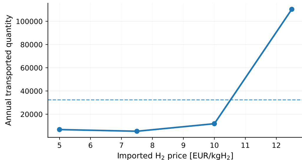
H 2 network throughput
