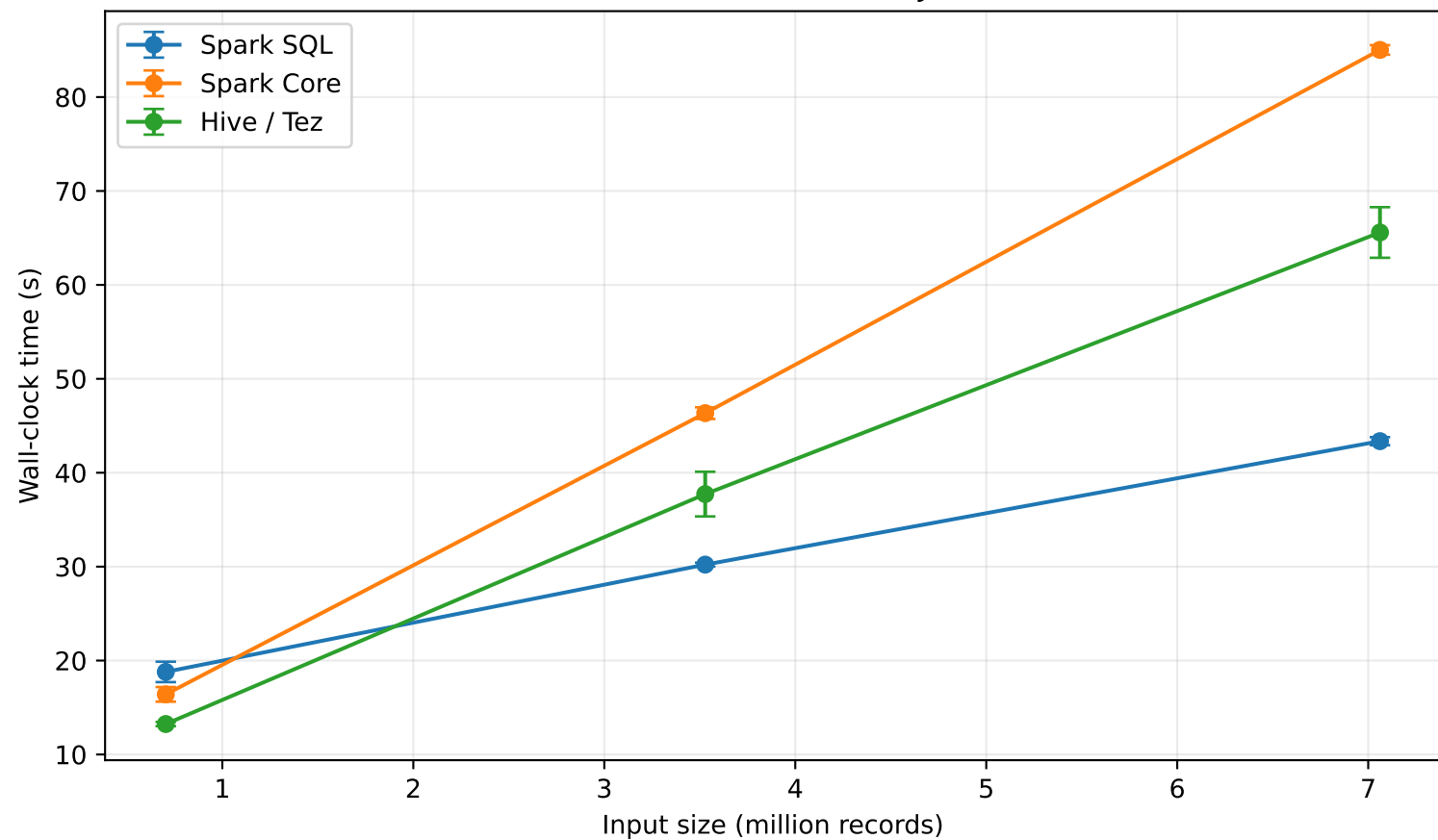
Local execution time — Job 2
