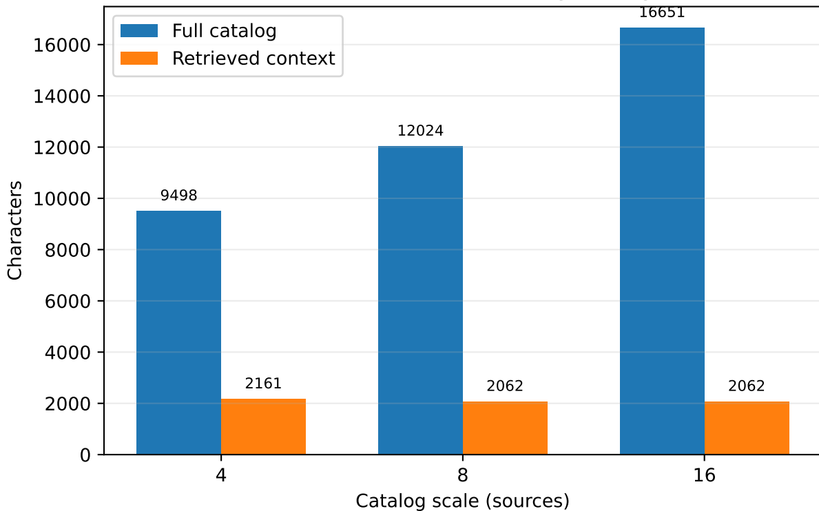
Context size under catalog scaling
