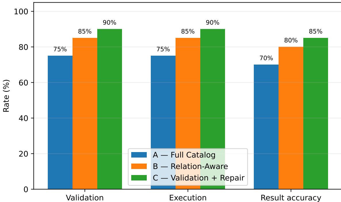
Held-out Text-to-Spark-SQL performance
