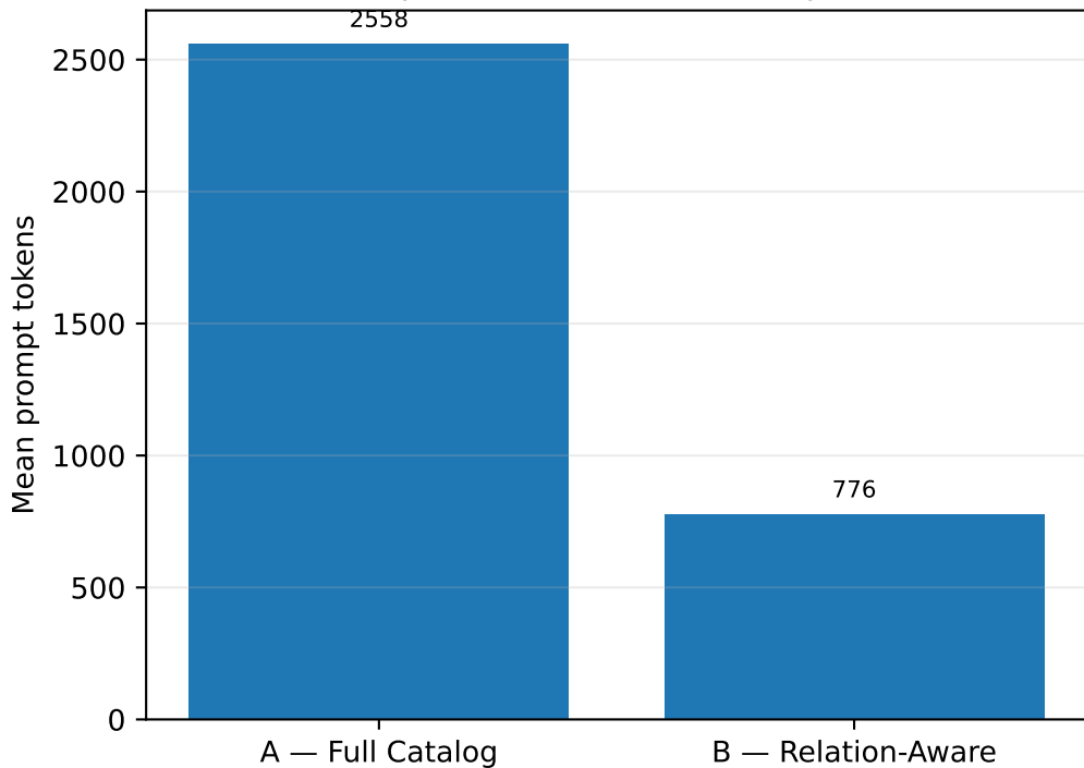
Prompt size on 20 held-out queries
