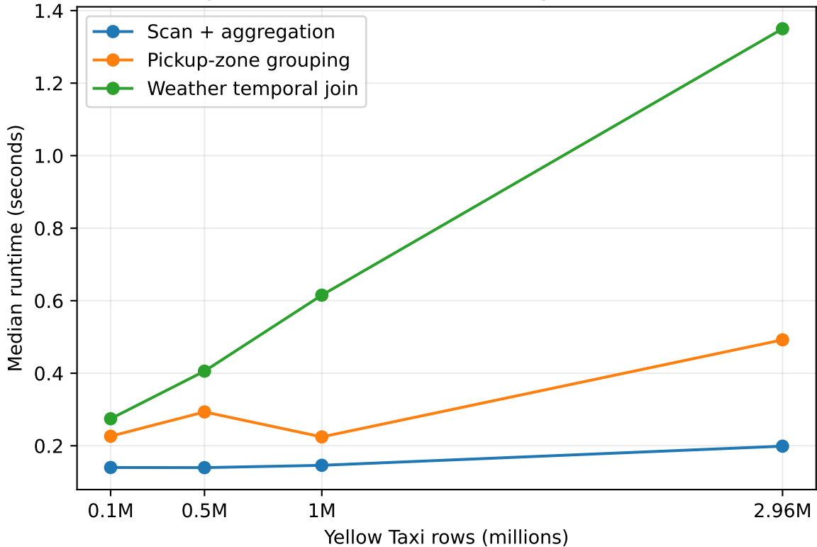
Spark runtime under increasing data volume
