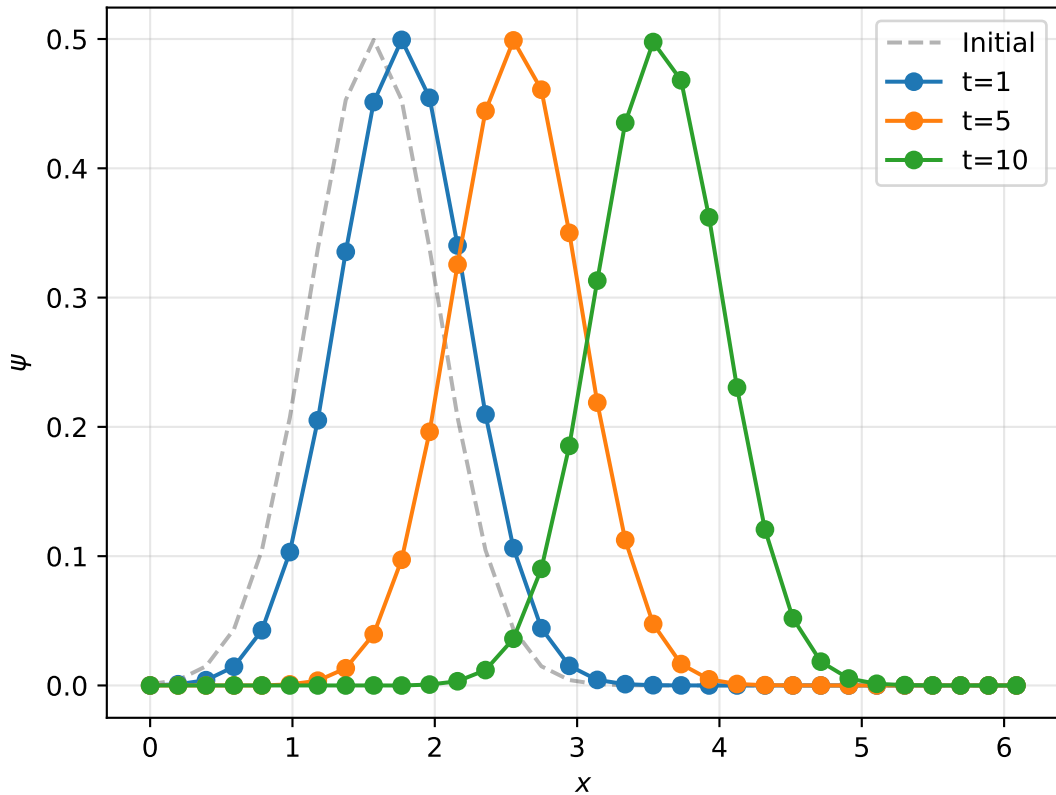
Pure Advection (Gaussian), c=0.2
