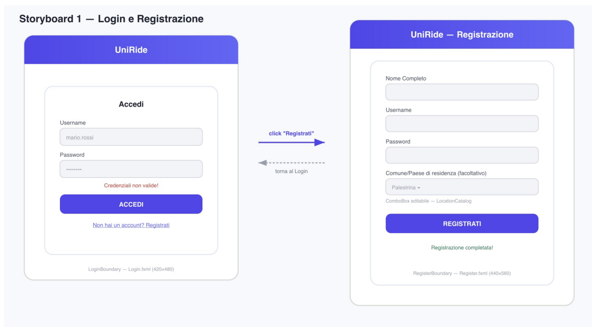
Mockup 1 — Storyboard Login e Registrazione (LoginBoundary / RegisterBoundary)
