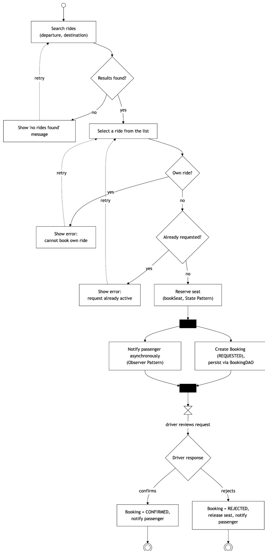
Figure 9 — Activity diagram of the main application flow
