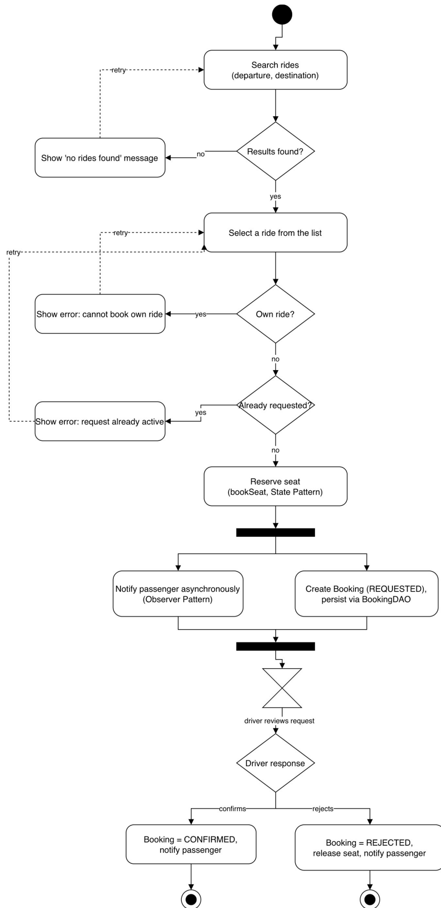
Figure 9 — Activity diagram of the main application flow
