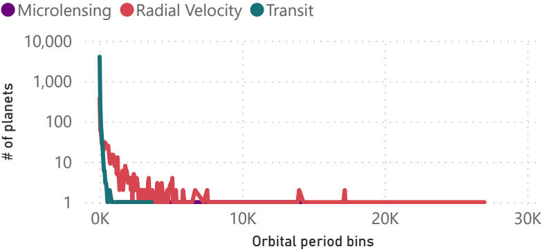
Number of planets per orbital periods
