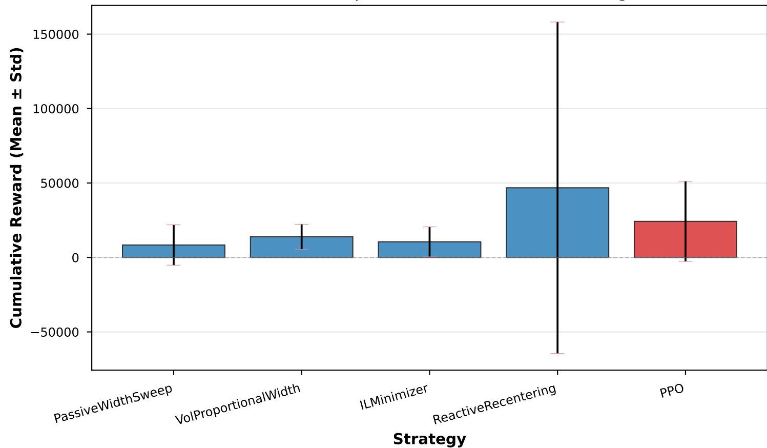
Performance Comparison: PPO vs. Baseline Strategies
