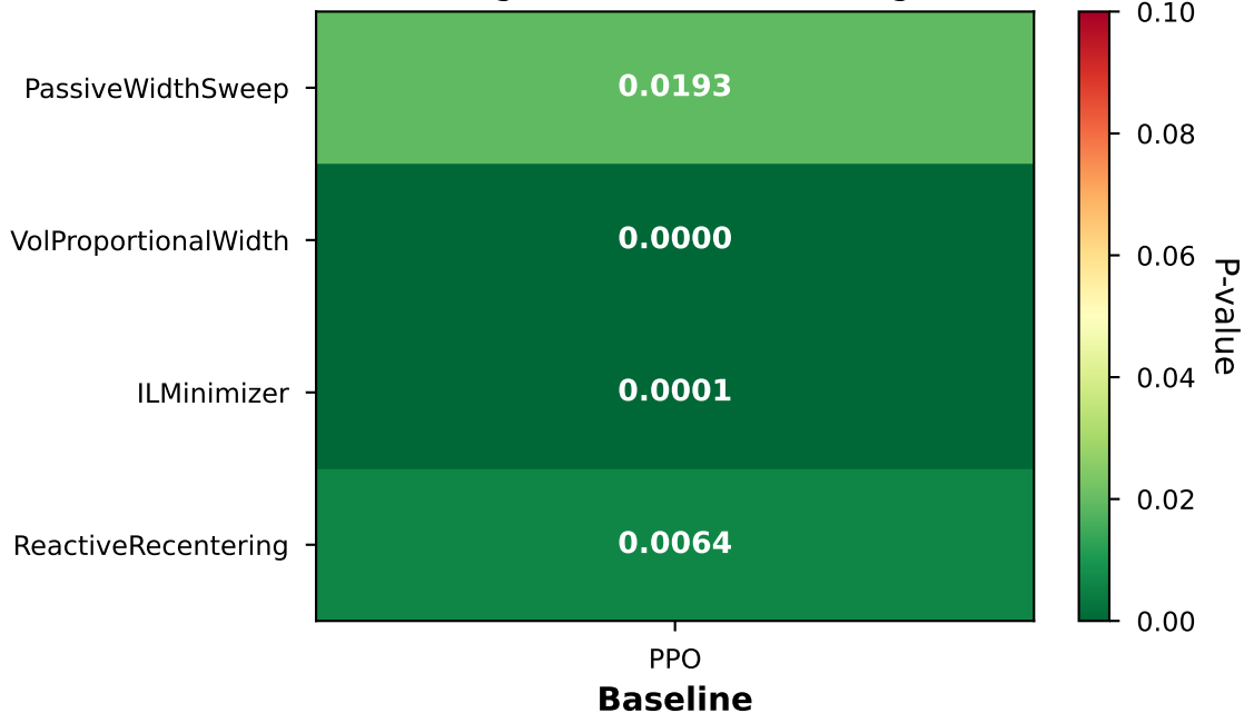
P-values: Strategy vs. PPO (Green = significant, Red = not significant)
