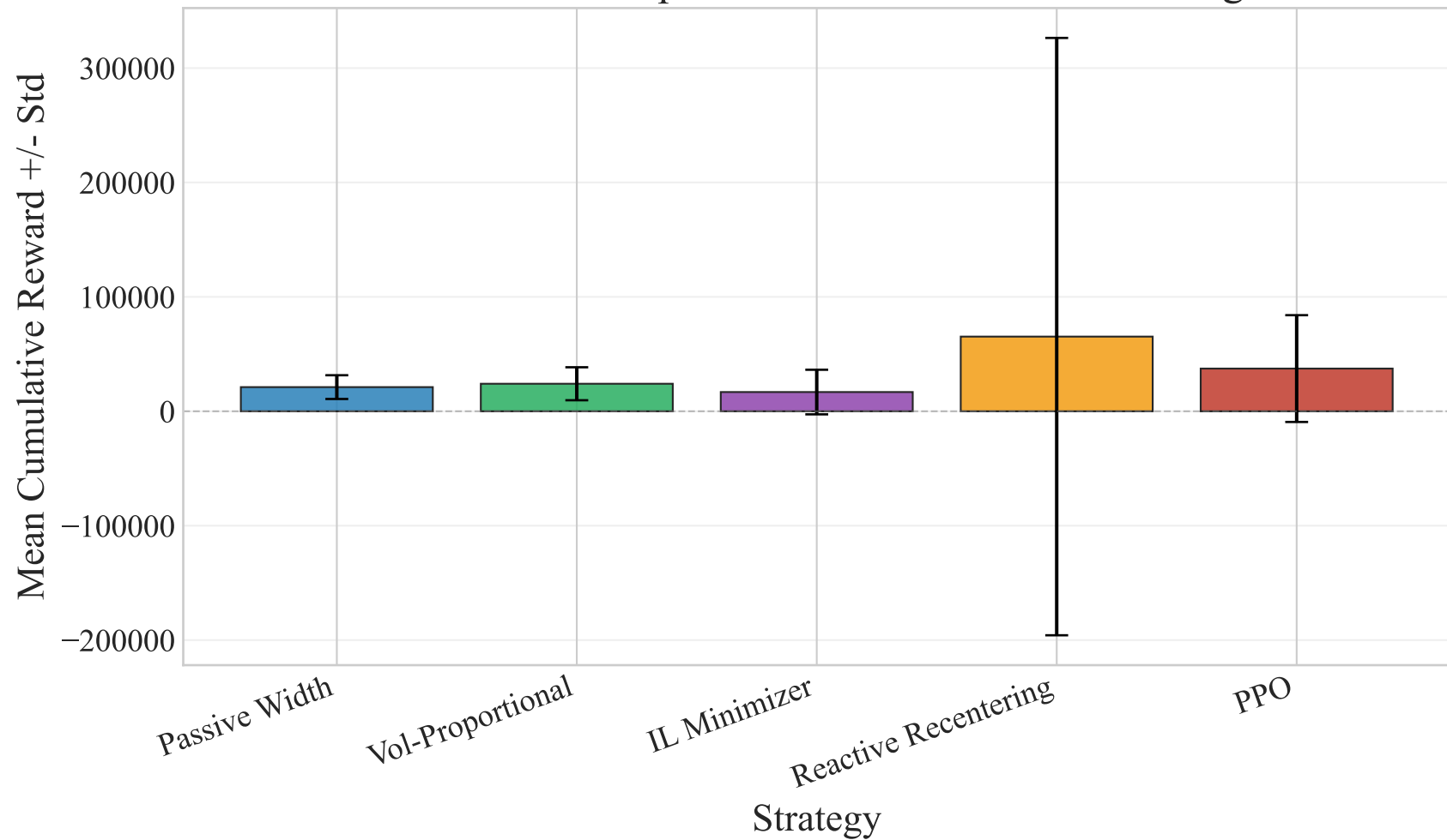
Performance Comparison: PPO vs. Baseline Strategies
